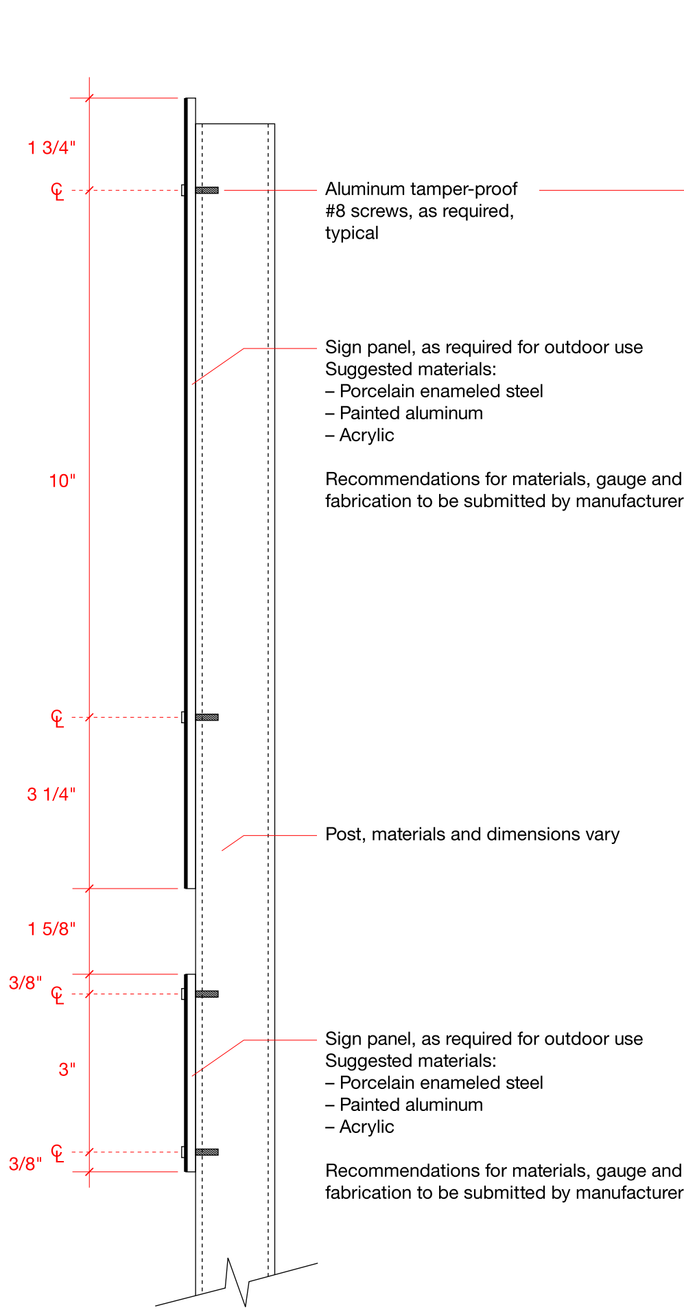
Side Section View
